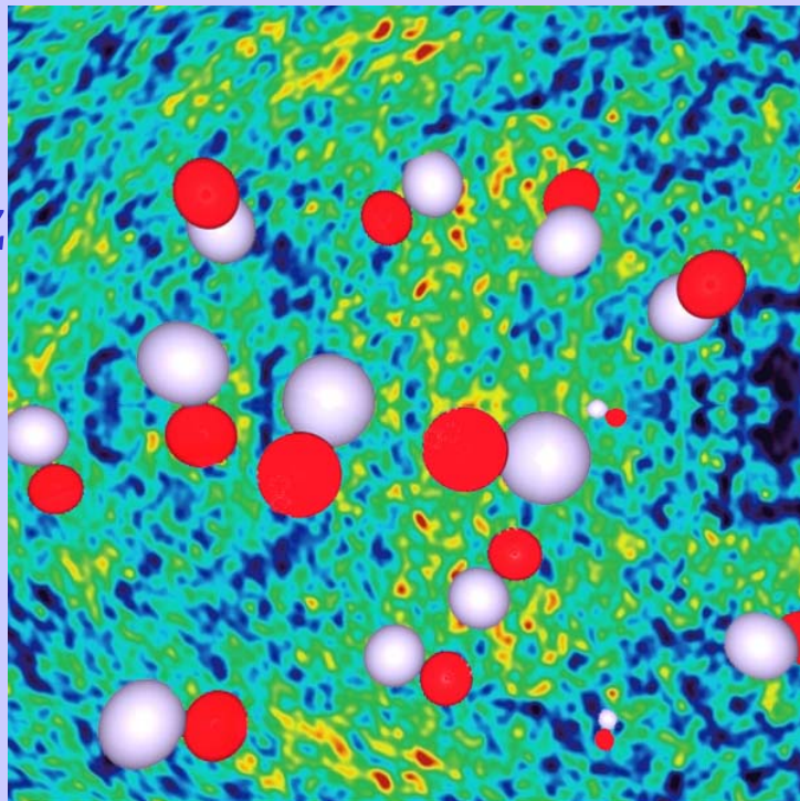
Primordial molecules on WMAP-detail
