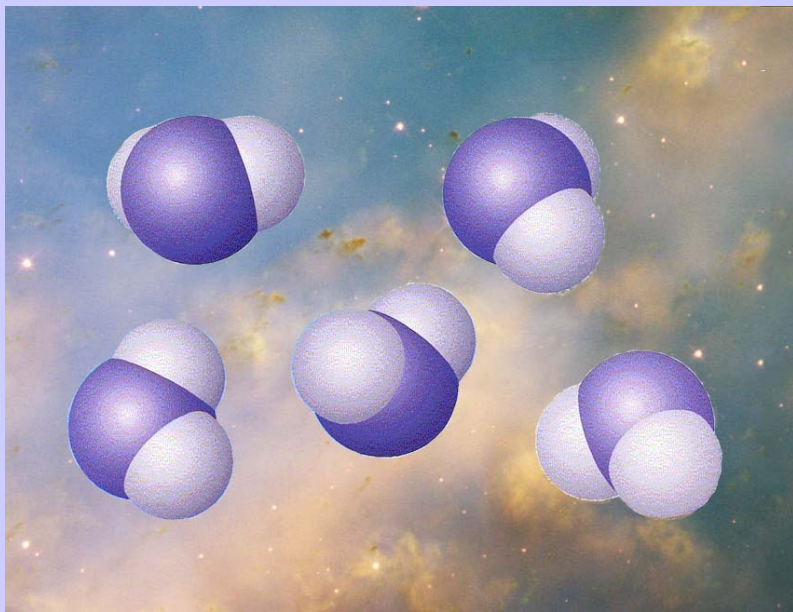
H 2 O on M27, Dumbell, HST
