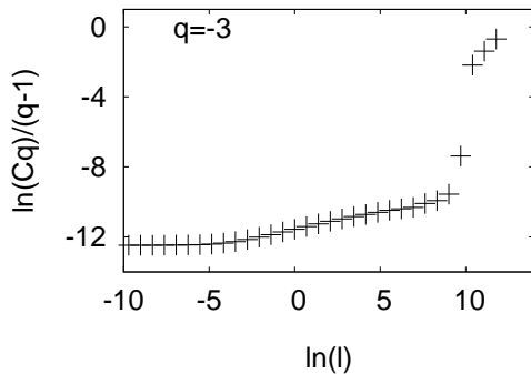
Fig. 2. \ln(C_q)/(q - 1) function of \ln(l) for q = -3 at time 13. A scaling range could be observed, for \ln(l) \in [-2.8; 6.2] .
