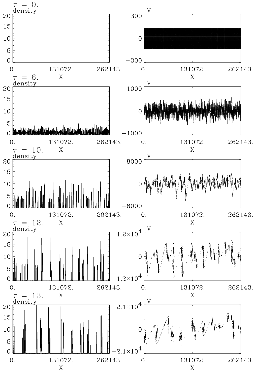
Fig. 1. Density and representation in mu -space for \tau = 0, 6, 10, 12 and 13 for a system of 262143 particles. The units are such that the length of the system is \sim 3547 Jean's length with \sim 74 particles by Jean's length.
