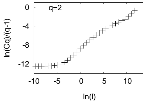
Fig. 3. \ln(C_q)/(q - 1) function of \ln(l) for q = 2 . Two scaling ranges could be observed, the first one for \ln(l) \in [-2.8; 2.1] , called SC1 hereafter, the second one for \ln(l) \in [2.1; 6, 2] , called SC2 hereafter.
