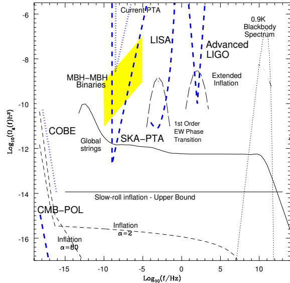
Figure 2. Summary of the potential cosmological sources of a stochastic gravitational background, including inflationary models, first-order phase transitions and cosmic strings and a primordial 0.9K black-body graviton spectrum as presented Battye & Shellard (1996). We also overlay bounds from COBE, from current millisecond pulsar timing and the goals from CMB polarization, LISA and Advanced LIGO (see e.g. Maggiore 2000). The PTA provided by the SKA will improve on the current MSP limit by about four orders of magnitude. The gray area indicates the spectrum of an additional astrophysical background caused by the merger of massive black holes (MBHs) in early galaxy formation (e.g. Rajagopal & Romani 1995, Jaffe & Backer 2003). For this background, \Omega_{\text{gw}} \propto f^{2/3} , whilst its amplitude depends on the MBH mass function and merger rate. The uncertainty is indicated by the size of the shaded area.
