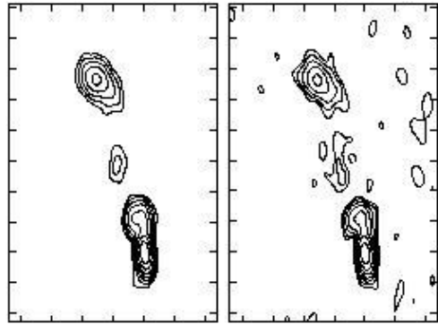
Fig 1: (left) A radio source image after calibration using two nearby calibrators, one 0.8^\circ to the east and another 3.2^\circ to the west. (right) The radio source image after calibration using only the nearer calibrator. The minimum contour level on both plots is 3 mJy and increase by a factor of 2. The tick marks are separated by 2 mas.
