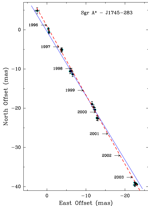
Fig 2: The motion of Sgr A*, measured with respect to the quasar J1745-283: The plotted points show the measured position and error estimate of the location of Sgr A* between 1996.3 and 2003.5. The dashed line shows the best fit to the proper motion, and the solid line shows the orientation of the galactic plane, arbitrarily aligned with Sgr A* in 1999.6. The apparent motion of Sgr A* is produced by the solar motion around the galactic center, including the motion perpendicular to the galactic plane plus a residual motion which determines a lower mass limit of Sgr A*.
