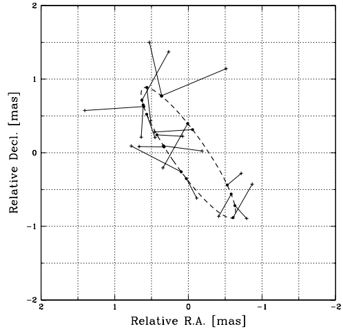
Fig 3: The Orbital Motion of HR8703: The dashed line shows the best fit orbital motion associated with HR8703 after removal of the parallax and proper motion based on 4 years of observation. The plotted crosses show the measured residual positions, and the dots show their expected location on the orbit with a 2.5-day period.
