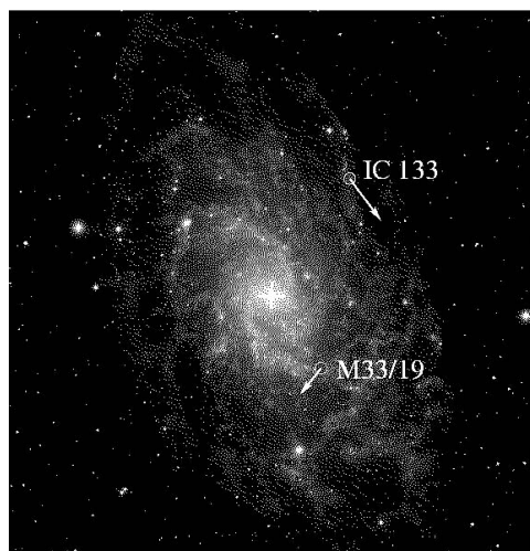
Fig 4: The Motion of Two Maser Sources in M33: The arrows show the expected motion of the maser source IC133 (100 km/s) and M33/19 (62 km/s) with respect to the radio core, derived from the known rotation model for the galaxy. The radio observations of the relative motion of the two maser sources were made over a 2.5 year period and give a distance uncertainty to M33 of 15%.
