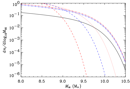
Figure 1. Predictions of the evolution in the HI mass function from AR2004. The dot-dashed lines show their ‘Model A’ at z = 1 (lower, blue) and z = 2 (upper, red) with the solid (black) line showing the measured local HI mass function (Zwaan et al. 2003). The dashed lines show their ‘Model B’ at z = 1 (right-most, blue) and z = 2 (leftmost, red), and the dotted lines their ‘Model C’ at z = 1 (upper, blue) and z = 2 (lower, red).
