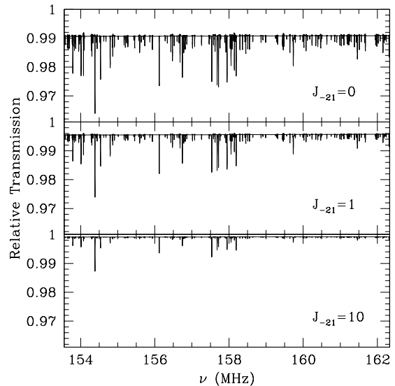
Figure 4. Simulated spectra for HI 21cm absorption by mini-halos at z = 9 . The different frames show the expected absorption for different values of the extragalactic Ly \alpha radiation field J_{-21} , in units of 10^{-21} erg s ^{-1} cm ^{-2} Hz ^{-1} sr ^{-1} [10].
