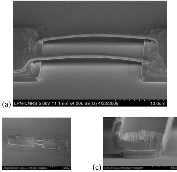
Fig.2 SEM pictures before passivation. (a) Air-bridges and the pair of anodes. (b) The 330GHz circuit. (c) Close-up of the T-Anode.
