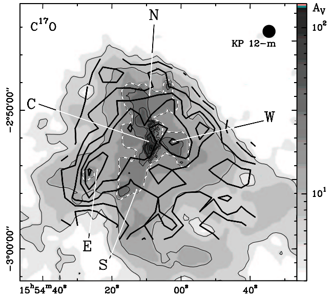
Fig. 4. same as Fig. 3 for C^{17}O (J:1-0). C^{17}O levels : 0.1 to 0.7 by 0.1 K km s^{-1} (r.m.s. \approx 30 mK km s^{-1} )
