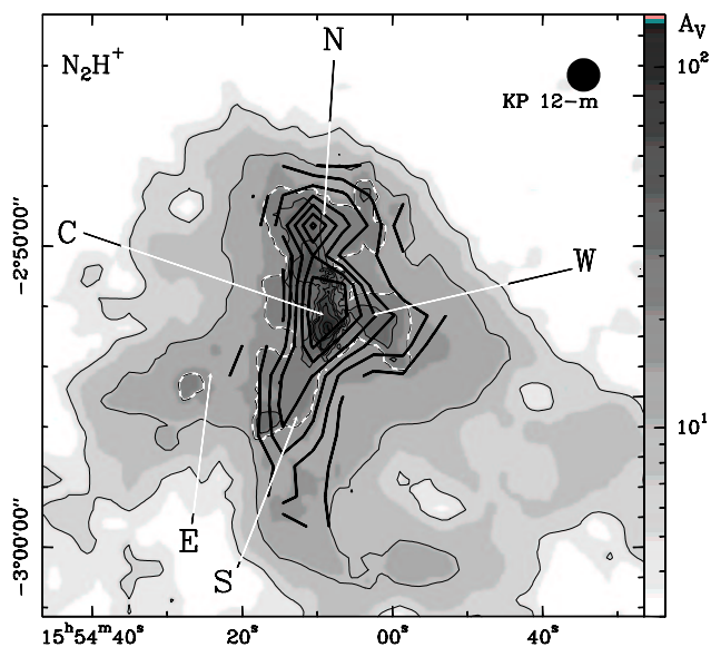
Fig. 7. same as Fig. 3 for \text{N}_2\text{H}^+ ( J:1-0 ). \text{N}_2\text{H}^+ levels : 0.4 to 2.8 by 0.4 \text{ K km s}^{-1} (r.m.s. \approx 75 \text{ mK km s}^{-1} )
