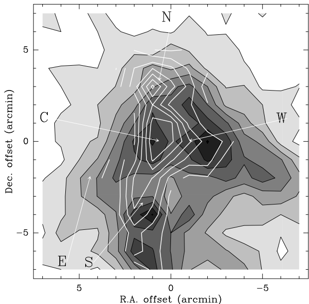
Fig. 14. ^{32}\text{SO} ( J_N:3_2-2_1 ) peak intensity (filled black contours) with \text{N}_2\text{H}^+ ( J:1-0 ) integrated intensity (grey contours) superimposed to it. Coordinates are offset from the reference position. ^{32}\text{SO} levels : 0.3 to 2.4 by 0.3 K. \text{N}_2\text{H}^+ levels : 0.4 to 2.8 by 0.4 \text{K km s}^{-1}
