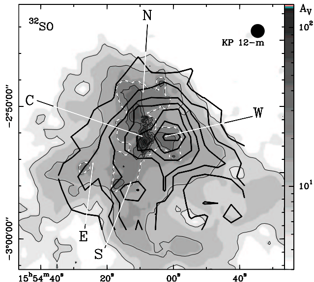
Fig. 6. same as Fig. 3 for ^{32}\text{SO} ( J_N:3_2-2_1 ). ^{32}\text{SO} levels : 0.3 to 2.1 by 0.3 \text{ K km s}^{-1} (r.m.s. \approx 60 \text{ mK km s}^{-1} )
