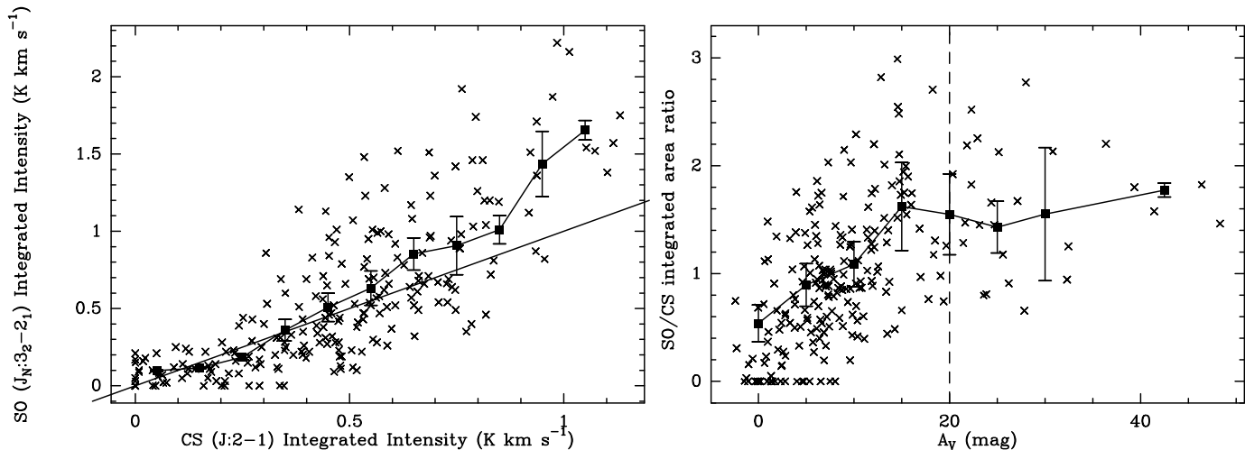
Fig. 15. left ^{32}\text{SO} ( J_N:3_2-2_1 ) integrated intensity cross-correlated with \text{C}^{32}\text{S} ( J:2-1 ) integrated intensity (KP 12-m data). Square symbols represent the average of the ^{32}\text{SO} values per 0.1 \text{ K km s}^{-1} \text{C}^{32}\text{S} intervals. Error bars represent the 1 \sigma dispersion. The straight line is the 1:1 slope. right ^{32}\text{SO} ( J_N:3_2-2_1 )/ \text{C}^{32}\text{S} ( J:2-1 ) integrated intensity ratio cross-correlated with A_V data degraded to 1' resolution. Square symbols represent the average of the SO/CS ratio per 5 mag intervals, except the last symbol which is the average of all the 5 points above A_V = 32.5 mag
