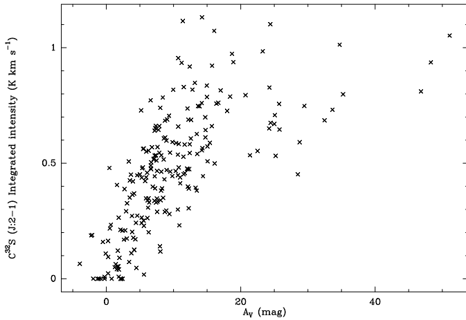
Fig. 12. C^{32}S (J:2–1) integrated intensity (KP 12-m data) cross-correlated with A_V data degraded to 1' resolution
