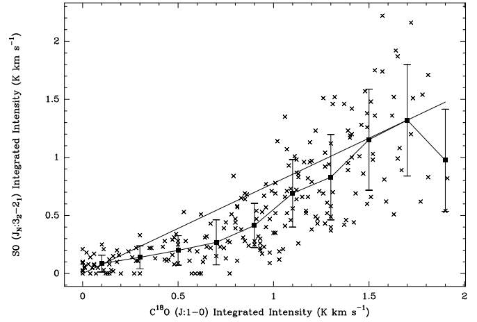
Fig. 13. ^{32}SO ( J_N:3_2-2_1 ) and C^{18}O (J:1–0) integrated intensity cross-correlation. KP 12-m data only. Square symbols represent the average of the ^{32}SO values per 0.2 \text{ K km s}^{-1} C^{18}O intervals. Error bars represent the 1 \sigma dispersion. The straight line goes through the origin to the 9th average value, its slope is 0.78
