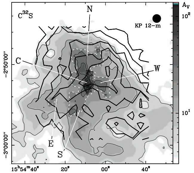
Fig. 5. same as Fig. 3 for C^{32}S (J:2-1). C^{32}S levels : 0.1 to 1.1 by 0.2 K km s^{-1} (r.m.s. \approx 45 mK km s^{-1} )
