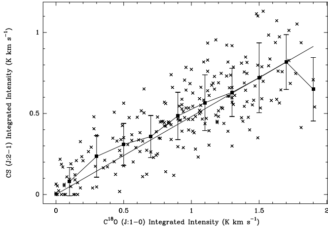
Fig. 11. C^{32}S (J:2–1) and C^{18}O (J:1–0) integrated intensity cross-correlation. KP 12-m data only. Square symbols represent the average of the C^{32}S values per 0.2 \text{ K km s}^{-1} C^{18}O intervals. Error bars represent the 1 \sigma dispersion. The straight line goes through the origin to the 9th average value, its slope is 0.48
