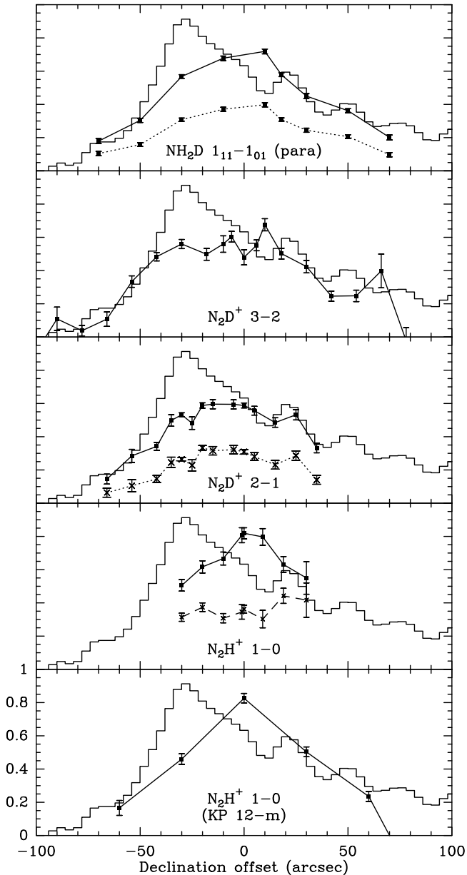
Fig. 9. North-south cut through the dust peak (R.A. offset = +30''). The histogram displays the 1.2 mm dust emission while the sets of dots trace N-bearing species through the peak. The vertical scales are all arbitrary. They are set to have the species integrated intensities proportional to the dust emission on the peak sides. Except when specified, all data come from the IRAM 30-m. For \text{NH}_2\text{D} and \text{N}_2\text{D}^+ ( J:2-1 ), we have also plotted the sum of all the optically thin hyperfine components (dotted lines and crosses) while for \text{N}_2\text{H}^+ ( J:1-0 ), we have plotted the only hyperfine component ( (J_{F_1F_2}:1_{11}-0_{01}) , dashed line and crosses) which remains optically thin ( \tau \leq 1 ) in this cut. Error bars are 1\sigma errors on the integrated intensities
