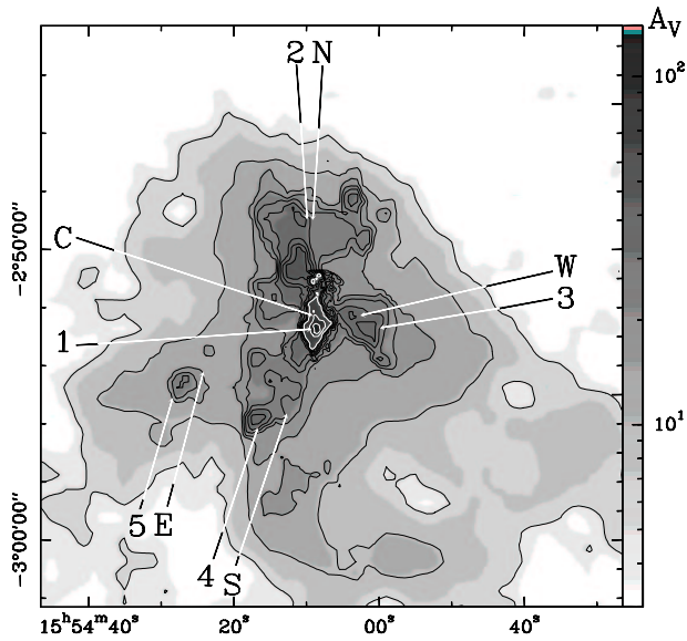
Fig. 2. Dust map from Paper II (in log grey scale). Coordinates are J2000 equatorial. Letters C, E, N, S, and W mark the molecular peaks while numbers 1 to 5 mark the corresponding dust peaks (see text). Dust peak #2 is not visible in this map but only in the dust emission map at 1.2 mm (see Paper II). Contours are from 5 to 50 by steps of 5 mag (black contours) and 60 to 120 by steps of 30 mag (white contours)
