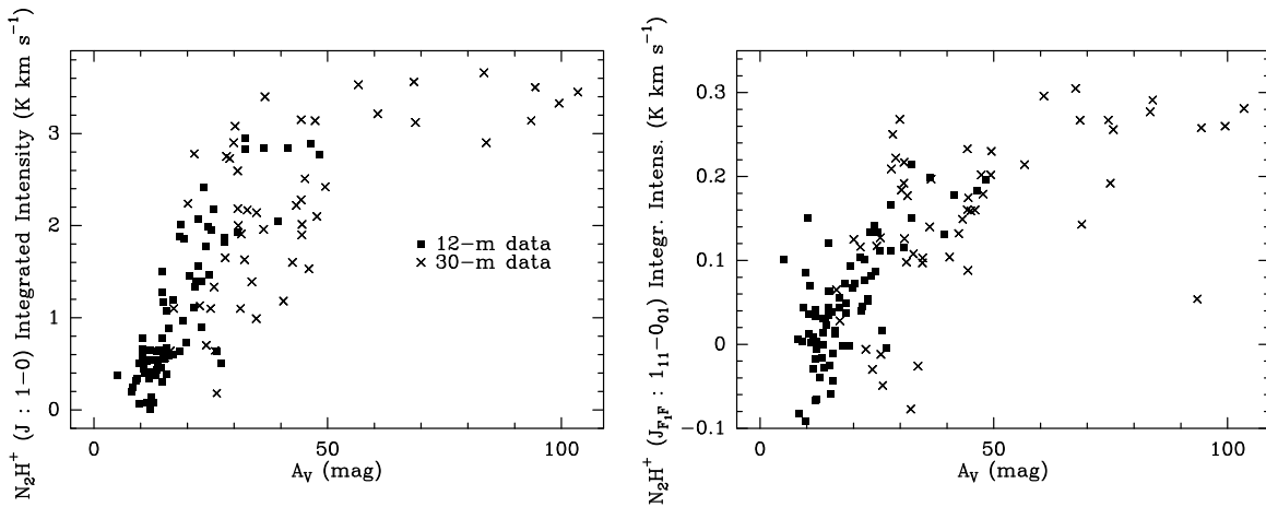
Fig. 16. ab \text{N}_2\text{H}^+ ( J:1-0 ) integrated intensity pixels cross-correlated with the A_V dust map pixels from Paper II. a (left) all seven hyperfine components have been included. b (right) only the weakest, optically thin ( J_{F_1F}:1_{11}-0_{01} ) component has been included. A_V map resolution is degraded to 1' for KP 12-m data and to 23'' for IRAM 30-m data
