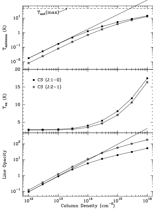
Fig. A.2. Same as Fig. A.1 except T_{\text{kin}} = 50 K
