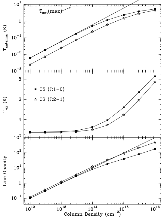
Fig. A.1. C^{32}S (J:1-0) and (J:2-1) transition properties as a function of column density. LVG model with T_{\text{kin}} = 10 K, \delta v = 1 km s ^{-1} and n = 10^3 cm ^{-3}
