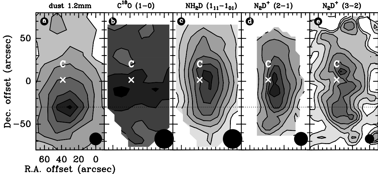
Fig. 8. a–e. IRAM 30-m maps of the molecular peak C and dust peak 1 (see paper II and Dickens et al. 2000). a Dust peak emission measured at 1.2 mm. Levels are 9 to 24 by 3 MJy/Sr. b C^{18}O ( J:1-0 ) integrated intensity. Levels are 1.2 to 1.8 by 0.2 K km s -1 . c NH_2D ( J_{KK'}:1_{11}-1_{01} ) integrated intensity. Levels are 0.15 to 1.05 by 0.15 K km s -1 . d N_2D^+ ( J:2-1 ) integrated intensity. Levels are 0.2 to 1.4 by 0.2 K km s -1 . e N_2D^+ ( J:3-2 ) integrated intensity. Levels are 0.05 to 0.35 by 0.05 K km s -1 . The horizontal dashed line indicates where the dust peak should appear in declination for the maps of the different species and the cross marks the Dickens et al. (2000) molecular peak C. The black spots in the bottom right corners indicate the different map resolutions of the IRAM 30-m (from 11'' to 23''). R.m.s. is \approx 24 mK km s -1 for maps b and c, 40 mK km s -1 for map d and 28 mK km s -1 for map e
