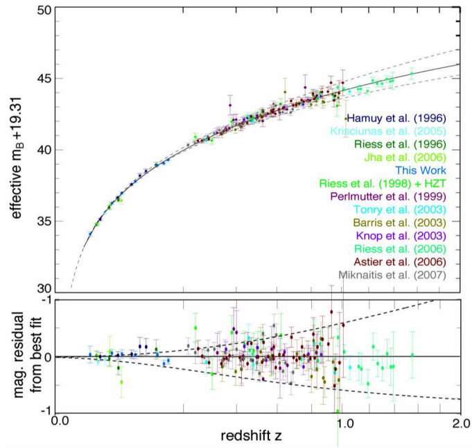
Figure 4.1: Comparison of SN data to different cosmological models (adapted from Kowalski, 2008, ApJ, 686,749). Full line is the best fit \Lambda CDM model. The bottom dashed line is Einstein - de Sitter model.
