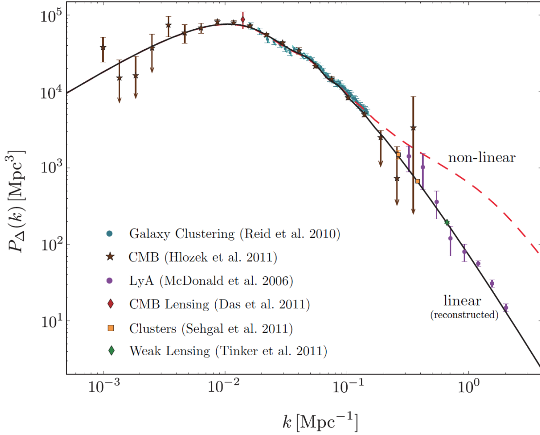
Figure 6.1: Compilation of recent observations of the matter power spectrum compared with theoretical prediction. Credit: D. Baumann, "Cosmology", Lecture notes. Reproduced with informal authorisation.
