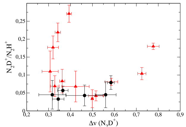
Fig. 6. FWHM of N_2D^+ 2-1 versus N_2D^+/N_2H^+ . Triangles are Perseus cores.
