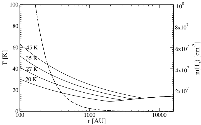
Fig. 9. Density (dashed line) and temperature (solid lines) profiles of the protostellar core models. The four temperature profiles represent models that yield values for T_{\text{Dust}} of 20 K, 27 K, 35 K and 45 K, respectively.
