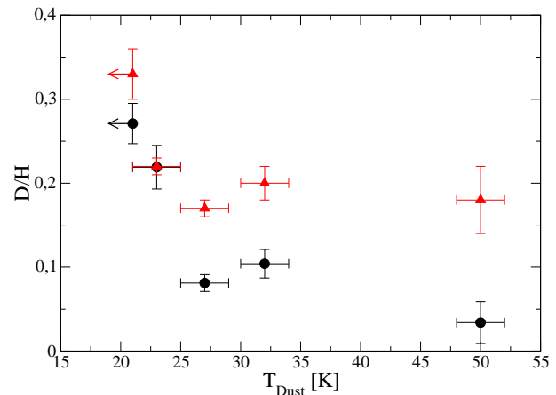
Fig. 8. Deuterium fractionation of NH_3 (red triangles) and N_2H^+ (black circles) versus dust temperature.
