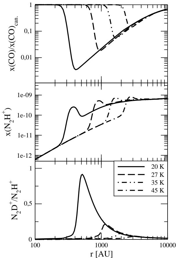
Fig. 11. The relative abundance of CO (upper panel), N_2H^+ (middle panel) and the N_2D^+/N_2H^+ ratio are shown as a function of radius. It can be clearly seen that the radius at which CO starts to deplete, as well as the peak of the deuterium fractionation, shifts outwards with increasing temperature.
