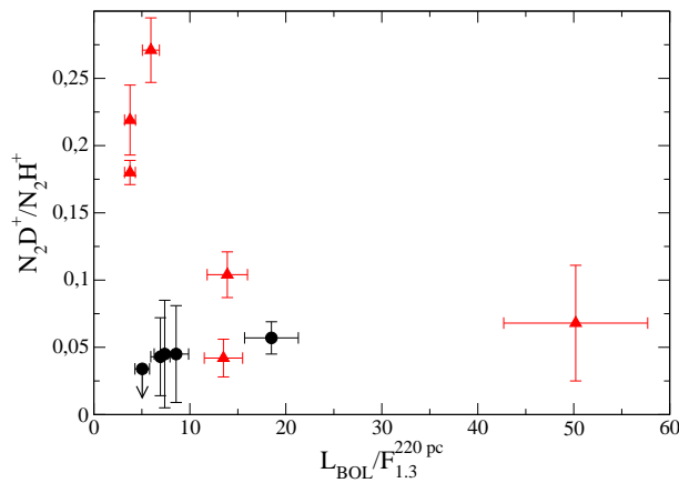
Fig. 5. N_2D^+/N_2H^+ versus L_{\text{BOL}}/F_{1.3}^{\text{D}_0} . All objects with high deuterium fractionation have low L_{\text{BOL}}/F_{1.3}^{\text{D}_0} ratios and are likely to be young objects. L 1527, which has one of the lowest L_{\text{BOL}}/F_{1.3}^{\text{D}_0} ratios, also has a quite upper limit on the N_2D^+/N_2H^+ ratio.
