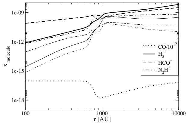
Fig. 12. The abundances of CO, H_3^+ , H_2D^+ , HCO^+ , DCO^+ , N_2H^+ , and N_2D^+ relative to H_2 are shown as a function of radius. The thick lines show the abundance profile of the protonated species. The thin lines show their singly-deuterated counterparts. These profiles apply to the model with T_{Dust} = 27 K.
