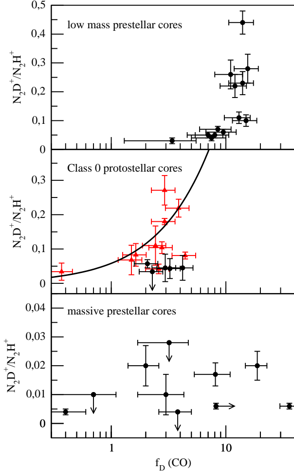
Fig. 4. N_2D^+/N_2H^+ column density ratio versus CO depletion factor for prestellar cores (upper panel, Crapsi et al. 2005), Class 0 protostars (middle panel, this work) and massive prestellar cores (lower panel, Fontani et al. 2006). The protostellar objects marked with triangles are located in the Perseus cloud. Among the Perseus objects, f_D(\text{CO}) and the deuterium fraction appear correlated. The solid curve in the middle panel is the result of fitting the sub-sample of Perseus cores with a formula adopted from Caselli et al. (1998, see text).
