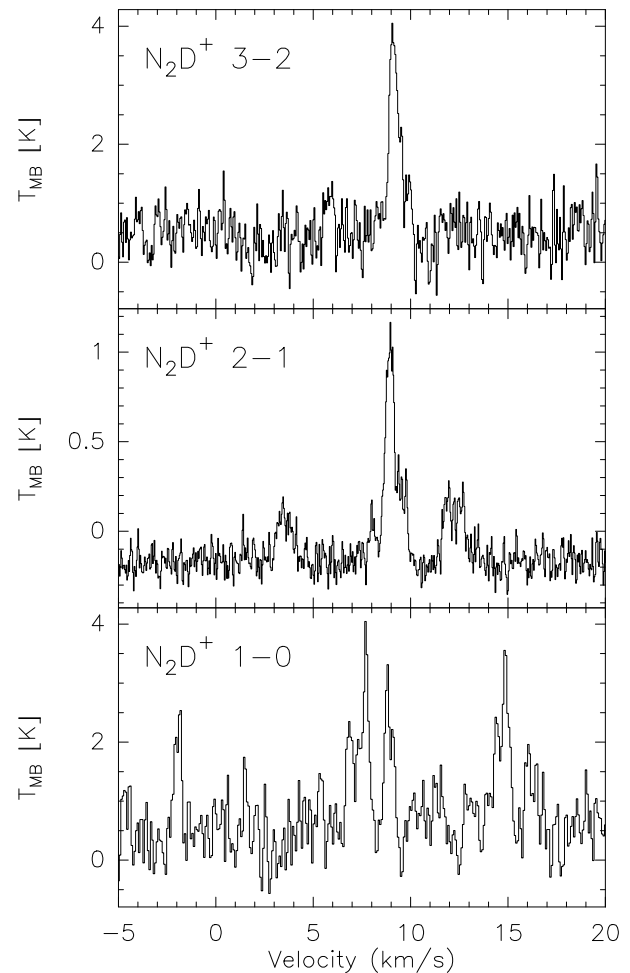
Fig. 1. Spectra of N_2D^+ 1-0, N_2D^+ 2-1 and N_2D^+ 3-2 toward HH 211, one of the youngest sources in our sample.
