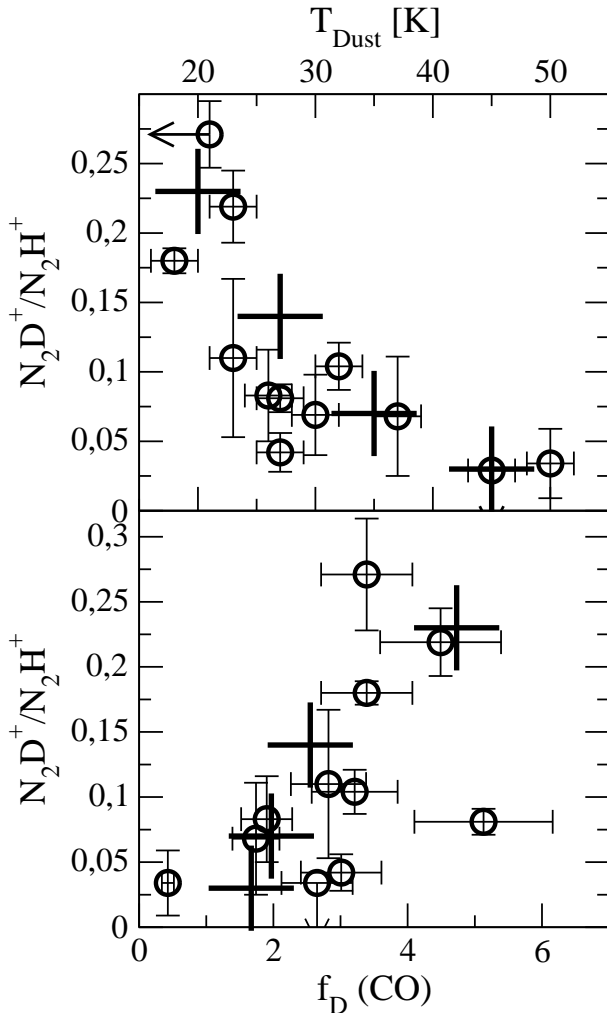
Fig. 10. Upper panel: N_2D^+/N_2H^+ ratio versus dust temperature. Lower panel: N_2D^+/N_2H^+ ratio and the CO depletion factor f_D(\text{CO}) . The open circles are the observed values for the sub-sample of cores in the Perseus cloud; the crosses are the model results. The N_2D^+/N_2H^+ ratio of the models was determined using the CTEX method.
