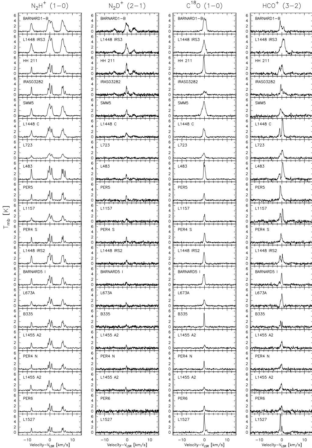
Fig. 2. Spectra of N_2H^+ 1-0, N_2D^+ 2-1, C^{18}O 1-0 and HCO^+ 3-2 (from left to right) of all 20 protostars of our sample. To be able to plot all spectra in one plot we divided the intensities of HCO^+ by three.
