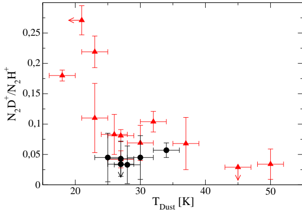
Fig. 3. Deuterium fractionation ( N_2D^+/N_2H^+ column density ratio) versus dust temperature. The largest N_2D^+/N_2H^+ ratios are seen at the lowest temperatures. As T_{\text{Dust}} increases, the deuterium fractionation declines. The objects marked with triangles are located in the Perseus cloud.
